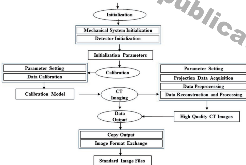
Fig. 2 Software workflow
